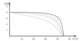
Schematic view of shadowing impact
