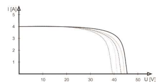
Schematic view of temperature impact
