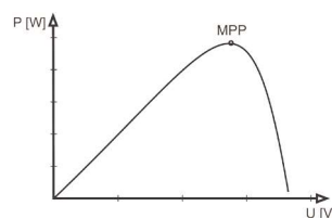
Schematic view of maximum power characteristic
